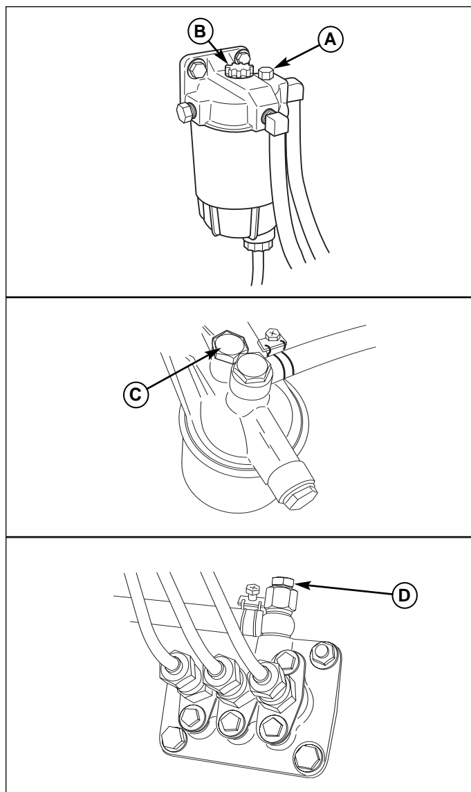
Figure 5. Fuel System Priming
